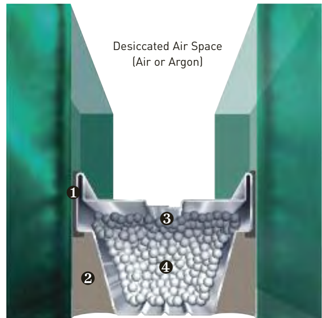
Double-Pane
